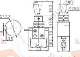
SPST 3P ON-OFF(LED) 20A 12VDC
