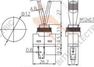
SPST 2P ON-OFF 20A 12VDC
