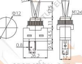
SPST 2P ON-OFF 20A 12VDC
