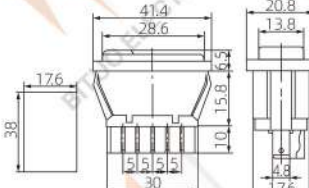
DPDT 5P(LED) 20A 12VDC
