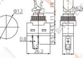
SPST 2P ON-OFF 20A 12VDC
