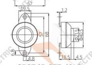
SPST 2P OFF-(ON) 30A 30VDC
