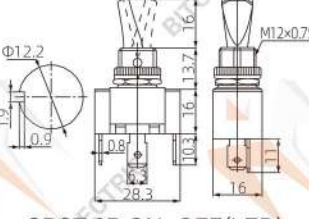
SPST 3P ON-OFF(LED) 30A 12VDC
