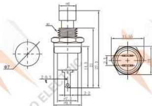
0.5A 250VAC
